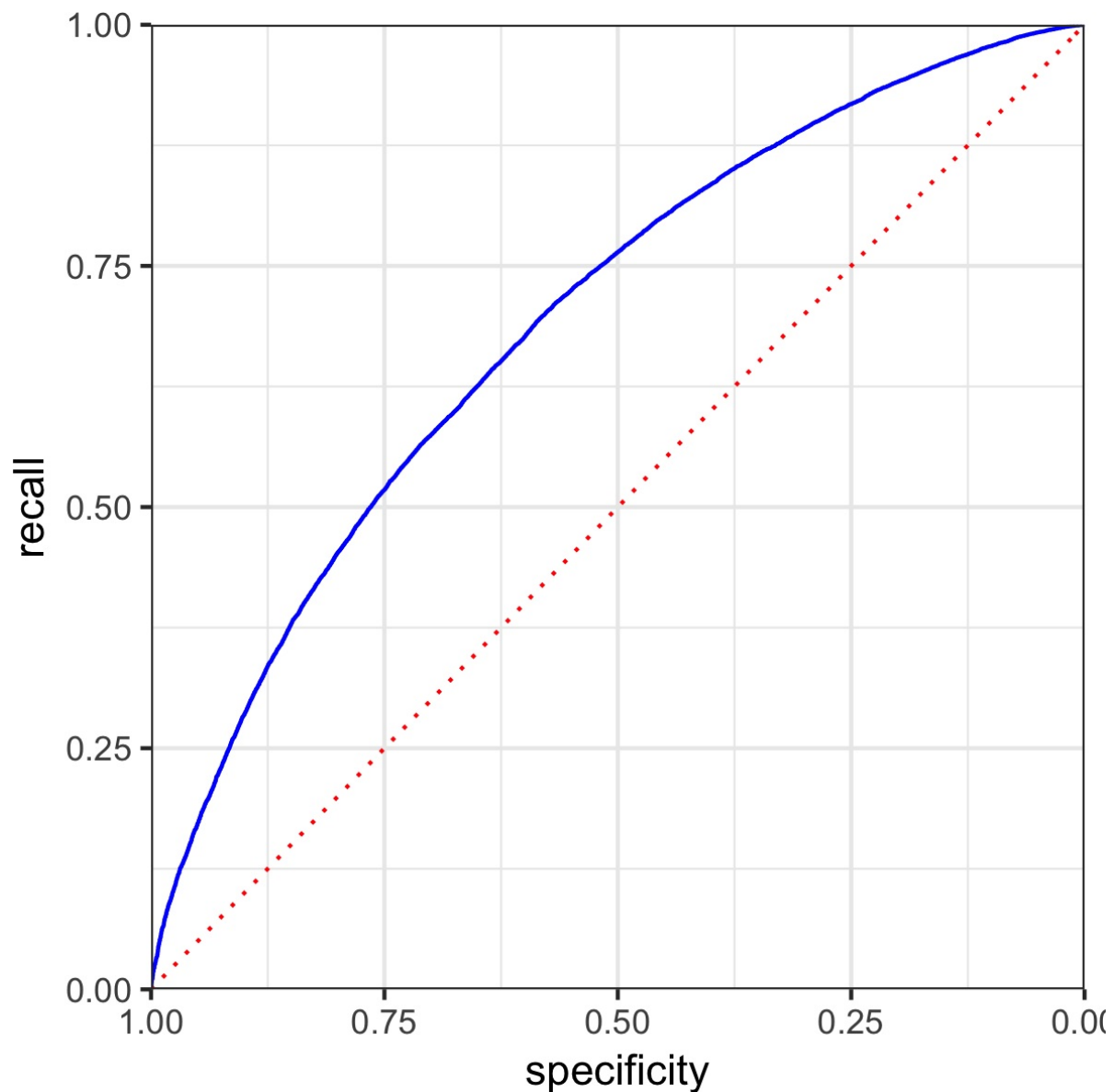
Figure 5-6. ROC curve for the loan data
