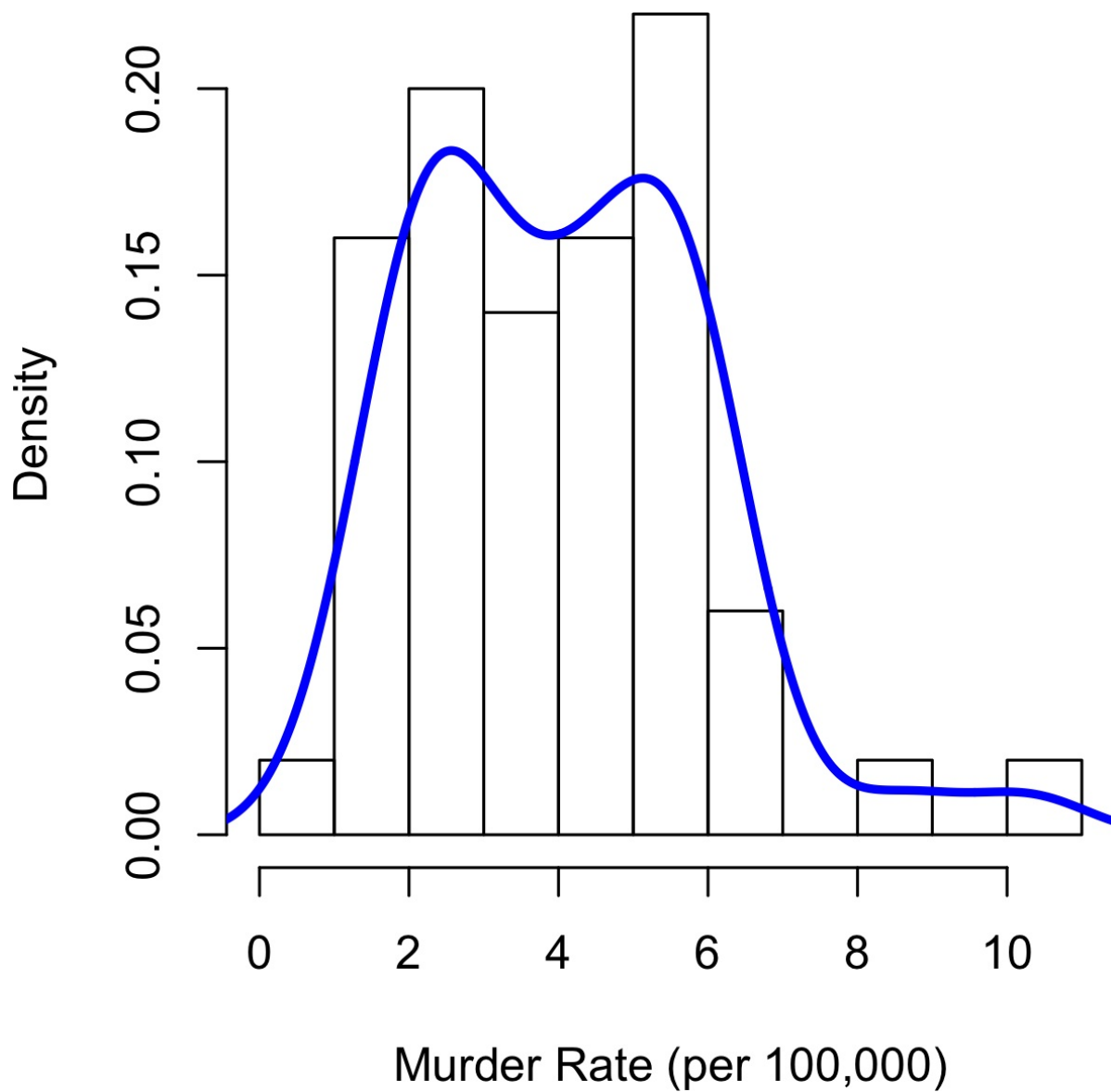
Figure 1-4. Density of state murder rates
