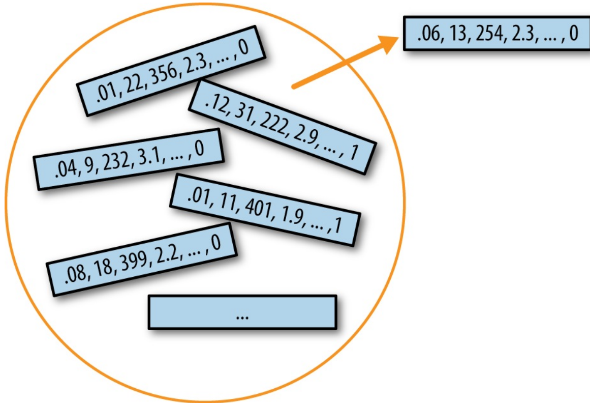
Figure 2-8. Multivariate bootstrap sampling
