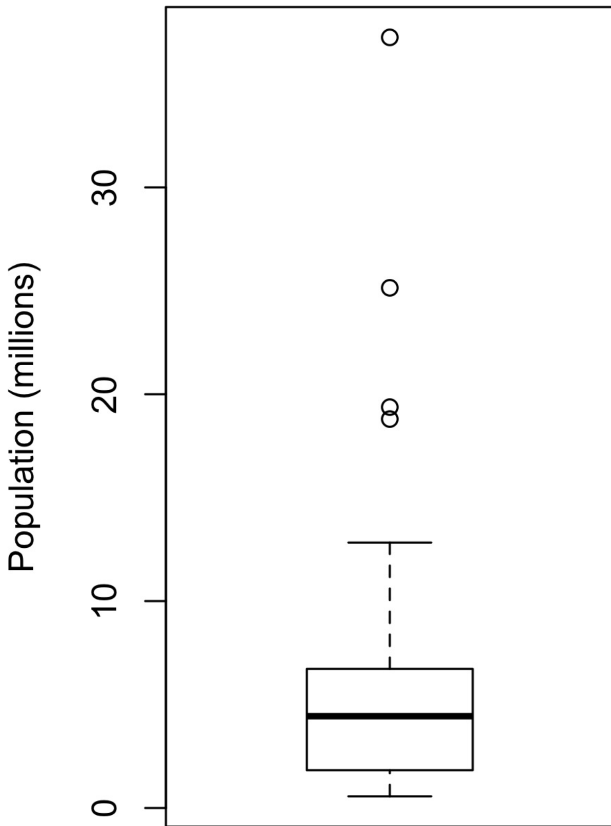
Figure 1-2. Boxplot of state populations
