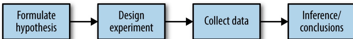
Figure 3-1. The classical statistical inference pipeline
