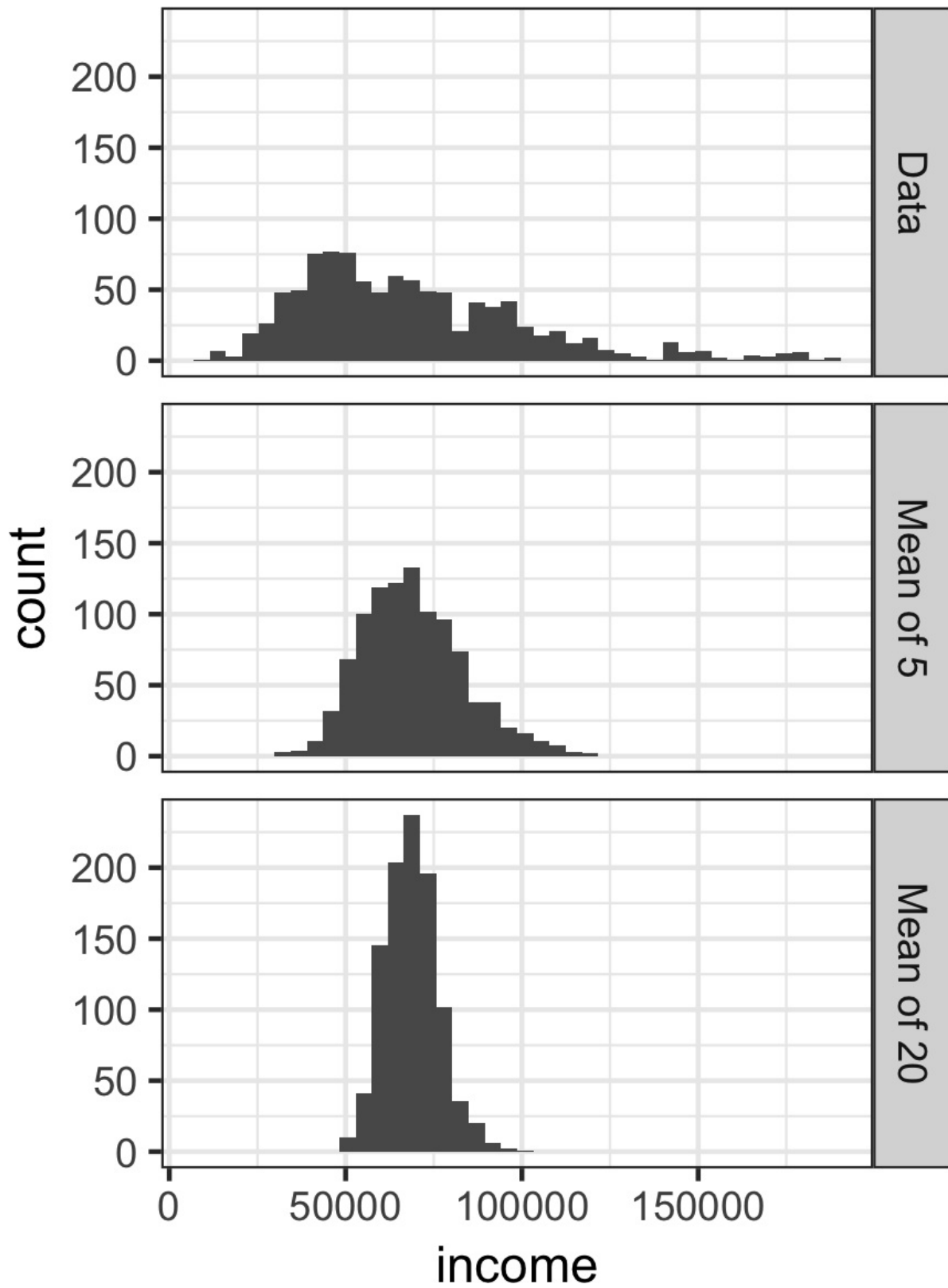
Figure 2-6. Histogram of annual incomes of 1,000 loan applicants (top), then 1000 means of n=5 applicants (middle), and n=20 (bottom)
