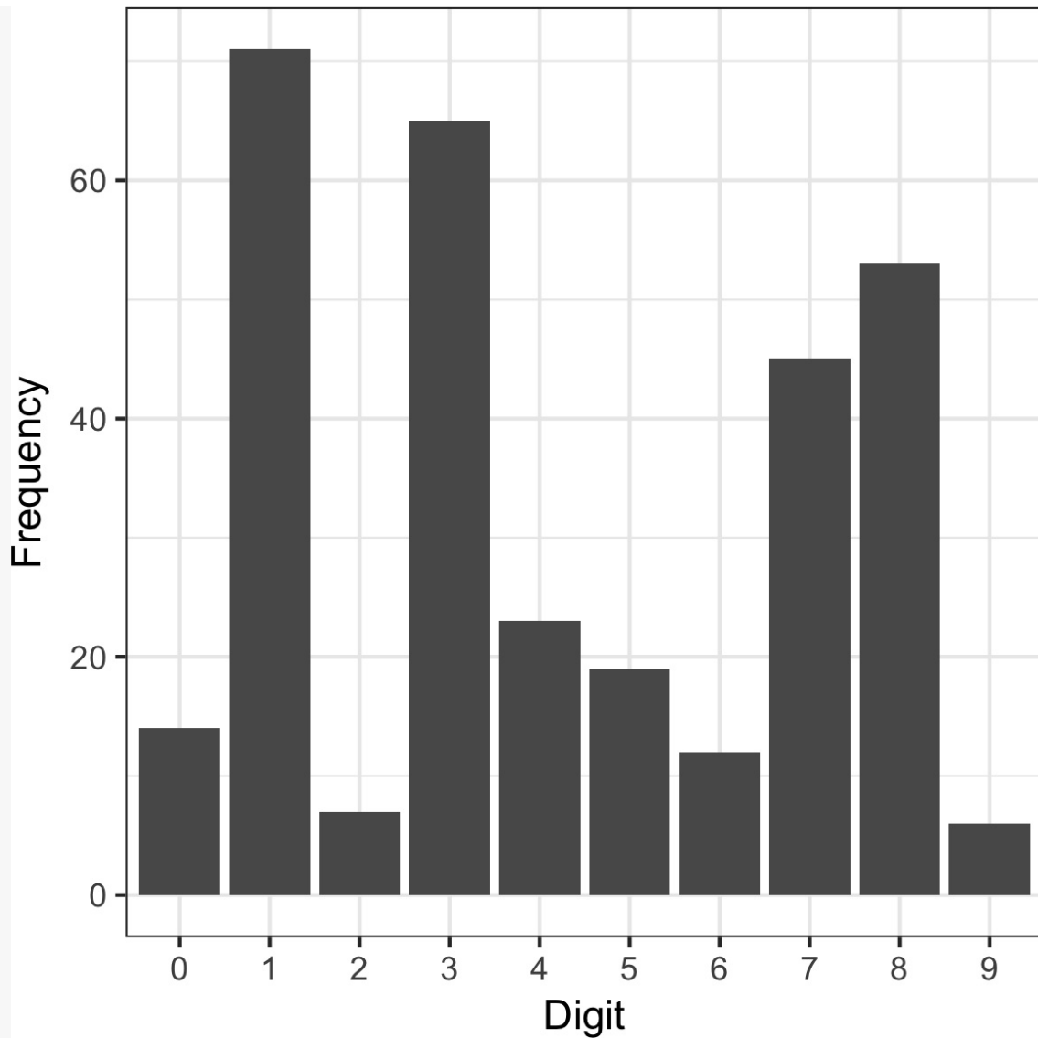
Figure 3-8. Frequency histogram for Imanishi-Kari lab data
